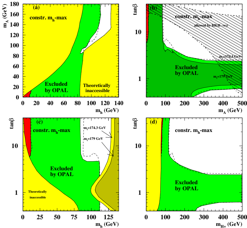
Fig. 18. Results for the constrained m_h\text{-max} benchmark scenario described in the text of Sect. 7.1. See Fig. 14 for the notation. The differently shaded regions in b show the exclusion for different values of m_{\text{top}} , as written in the Plot. The upper limit on m_h for different values of m_{\text{top}} is shown in c , as also expressed in the plot
