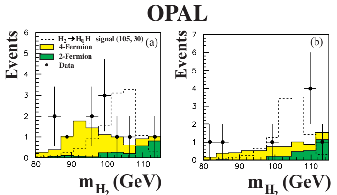
Fig. 4. Distributions of the reconstructed masses in the selection A and B of the missing energy channel for data taken at \sqrt{s} = 199 to 209 \text{ GeV} in the region 100 \text{ GeV} < m_{\mathcal{H}_2} < 110 \text{ GeV} (see Sect. 4.1.2)
