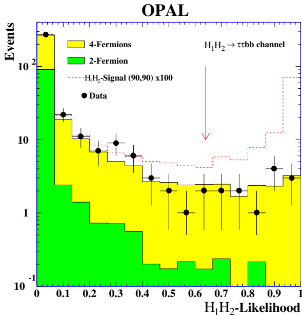
Fig. 11. Likelihood output of the e^+e^- \rightarrow \mathcal{H}_1\mathcal{H}_2 \rightarrow b\bar{b}\tau^+\tau^- search at 192–209 GeV. The arrow indicates the cut position. The signal is scaled with a factor of 100 with respect to a e^+e^- \rightarrow \mathcal{H}_1\mathcal{H}_2 \rightarrow b\bar{b}\tau^+\tau^- signal for \cos^2(\beta - \alpha) = 1
