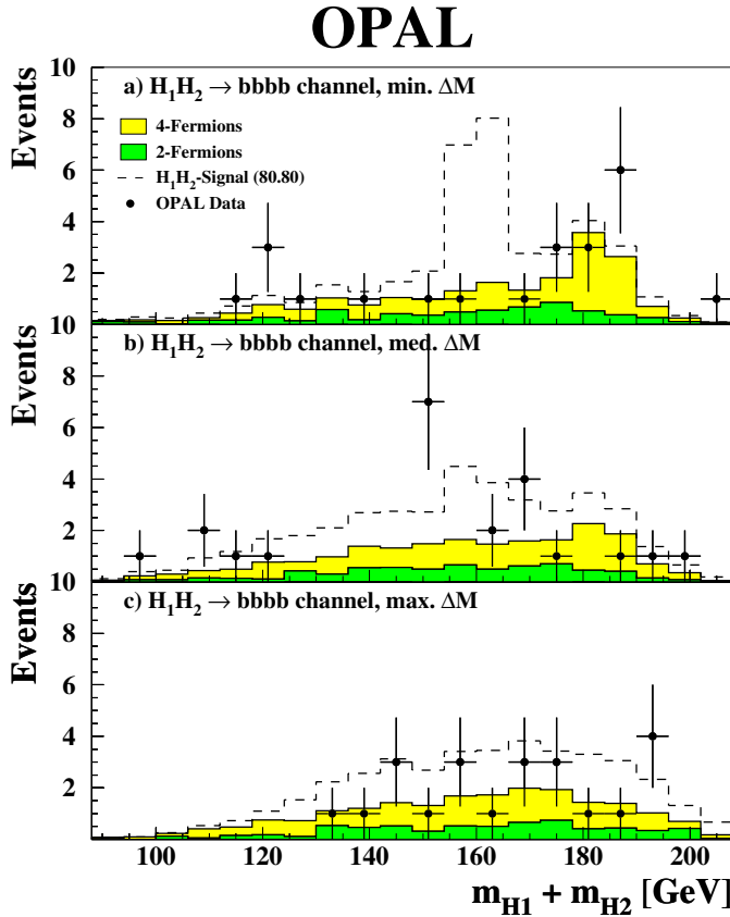
Fig. 8. Searches for e^+e^- \rightarrow \mathcal{H}_1\mathcal{H}_2 with high m_{\mathcal{H}_1} at 192–209 GeV. The sum of the reconstructed Higgs boson masses, m_{\mathcal{H}_1}^{\text{rec}} + m_{\mathcal{H}_2}^{\text{rec}} , for a the \mathcal{H}_1\mathcal{H}_2 \rightarrow 4b channel with the di-jet pairing combination which yields the smallest mass difference, \Delta M \equiv |m_{\mathcal{H}_2}^{\text{rec}} - m_{\mathcal{H}_1}^{\text{rec}}| , b the \mathcal{H}_1\mathcal{H}_2 \rightarrow 4b channel with the intermediate \Delta M combination, c the \mathcal{H}_1\mathcal{H}_2 \rightarrow 4b channel with the largest \Delta M combination. OPAL data are indicated by points with error bars, the four-fermion background by the light grey (yellow) histograms, and the two-fermion background by the darker grey (green) histograms. Shown as dashed histograms are the contributions expected from a Higgs boson signal with full strength at m_{\mathcal{H}_1} = m_{\mathcal{H}_2} = 80 GeV for a luminosity of 207 \text{ pb}^{-1} taken at \sqrt{s} = 199\text{--}209 GeV, added to the background expectation for a luminosity of 424 \text{ pb}^{-1} and the cross-section for \cos^2(\beta - \alpha) = 1
