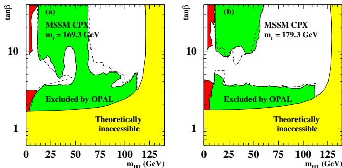
Fig. 24. The CPX MSSM 95%CL exclusion areas in the (m_{H_1}, \tan\beta) plane, using scans with a m_t = 169.3 GeV and b m_t = 179.3 GeV. Due to the change in the top masses a strong difference is observed compared to Fig. 23 c. See Fig. 14 for the notation
