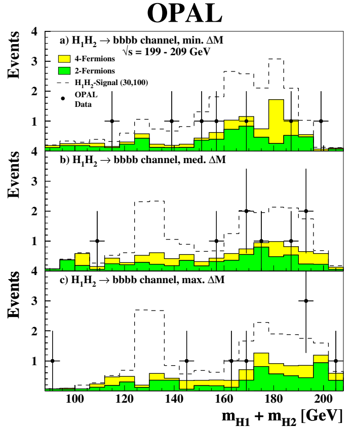
Fig. 9. Searches for e^+e^- \rightarrow \mathcal{H}_1\mathcal{H}_2 with low m_{\mathcal{H}_1} at 199–209 GeV. The sum of the reconstructed Higgs boson masses, m_{\mathcal{H}_1}^{\text{rec}} + m_{\mathcal{H}_2}^{\text{rec}} , for a the \mathcal{H}_1\mathcal{H}_2 \rightarrow 4b channel with the di-jet pairing combination which yields the smallest mass difference, \Delta M \equiv |m_{\mathcal{H}_2}^{\text{rec}} - m_{\mathcal{H}_1}^{\text{rec}}| , b the \mathcal{H}_1\mathcal{H}_2 \rightarrow 4b channel with the medium \Delta M combination, c the \mathcal{H}_1\mathcal{H}_2 \rightarrow 4b channel with the maximum \Delta M combination. OPAL data are indicated by points with error bars, the four-fermion background by the light grey (yellow) histograms, and the two-fermion background by the darker grey (green) histograms. Shown as dashed histograms are the contributions expected from a Higgs boson signal with m_{\mathcal{H}_1} = 30 GeV, m_{\mathcal{H}_2} = 100 GeV, added to the background expectation for a luminosity of 207 \text{ pb}^{-1} and the cross-section for \cos^2(\beta - \alpha) = 1
