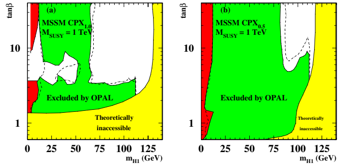
Fig. 28. The CPX MSSM 95 % CL exclusion areas in the (m_{H_1}, \tan\beta) plane, using scans a preserving the CPX ratios of \mu , A_{b,t} and m_{SUSY} , using m_{SUSY} = 1 TeV, and b m_{SUSY} = 1 TeV keeping \mu and A_{b,t} at their CPX values. See Fig. 14 for the notation
