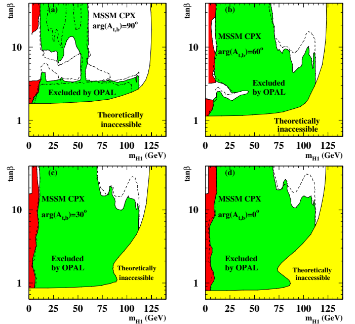
Fig. 25. The CPX MSSM 95%CL exclusion areas in the (m_{H_1}, \tan\beta) plane, using scans with a \arg(A_{t,b}) = \arg(m_{\tilde{g}}) = 90^\circ , b \arg(A_{t,b}) = \arg(m_{\tilde{g}}) = 60^\circ , c \arg(A_{t,b}) = \arg(m_{\tilde{g}}) = 30^\circ and d \arg(A_{t,b}) = \arg(m_{\tilde{g}}) = 0^\circ . While the CPV phases decrease, effects from CP violation like the strong H_2 \rightarrow H_1H_1 contribution vanish. See Fig. 14 for the notation
