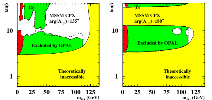
Fig. 26. The CPX MSSM 95%CL exclusion areas in the (m_{H_1}, \tan\beta) plane, using scans with a \arg(A_{t,b}) = \arg(m_{\tilde{g}}) = 135^\circ and b \arg(A_{t,b}) = \arg(m_{\tilde{g}}) = 180^\circ . See Fig. 14 for the notation
