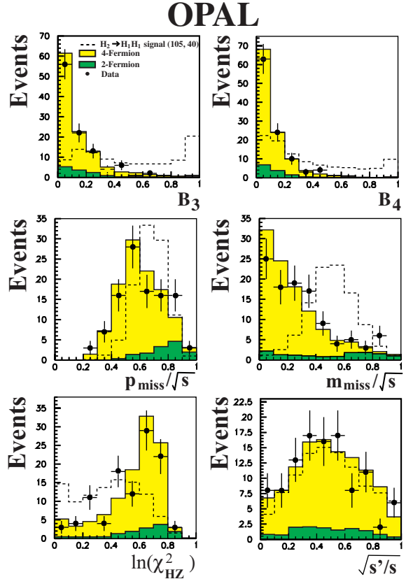
Fig. 2. Distributions of some ANN input variables for subsample B for e^+e^-\rightarrow\mathcal{H}_2Z\rightarrow b\bar{b}\nu\bar{\nu} and e^+e^-\rightarrow\mathcal{H}_1\mathcal{H}_1Z\rightarrow b\bar{b}b\bar{b}\nu\bar{\nu} (see Sect. 4.1.2) in the region 100 \text{ GeV} < m_{\mathcal{H}_2} < 110 \text{ GeV}
