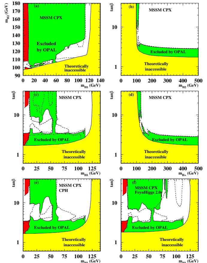
Fig. 23. The CPX MSSM 95% CL exclusion areas. Excluded regions are shown for a the (m_{H_1}, m_{H_2}) plane, b the (m_{H_2}, \tan\beta) plane, c the (m_{H_1}, \tan\beta) plane and d the (m_{H^\pm}, \tan\beta) plane. Figure e shows the (m_{H_1}, \tan\beta) of the CPH calculation alone, f shows the same projection of the FEYNHIGGS 2.0 calculation. See Fig. 14 for the notation. The dash-dotted line in c shows the area excluded on the 99.9% confidence level. In b and d the area excluded by Z width constraints or by decay independent searches is too small to be displayed
