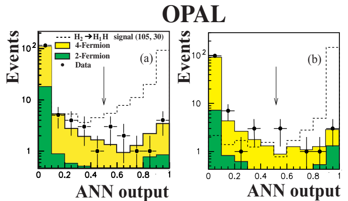
Fig. 3. Distributions of \text{ANN}_A a and \text{ANN}_B b in the dedicated selection for e^+e^- \rightarrow \mathcal{H}_2 Z \rightarrow b\bar{b}\nu\bar{\nu} and e^+e^- \rightarrow \mathcal{H}_1 \mathcal{H}_1 Z \rightarrow b\bar{b}b\bar{b}\nu\bar{\nu} (see Sect. 4.1.2) in the region 100 \text{ GeV} < m_{\mathcal{H}_2} < 110 \text{ GeV} . The arrows indicate the cut on the ANN output value
