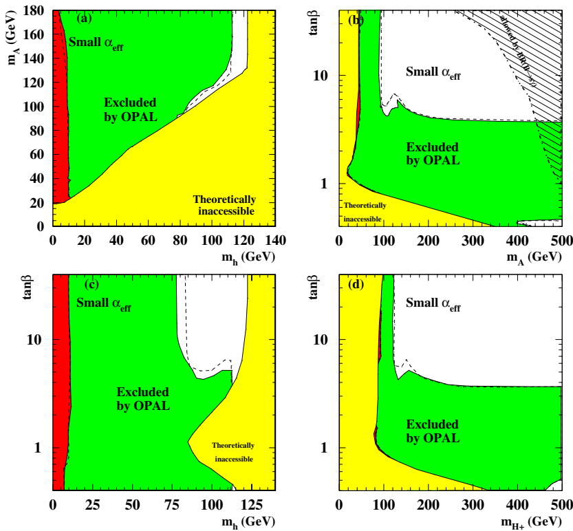
Fig. 21. Results for the small \alpha_{\text{eff}} benchmark scenario described in the text of Sect. 7.1. See Fig. 14 for the notation
