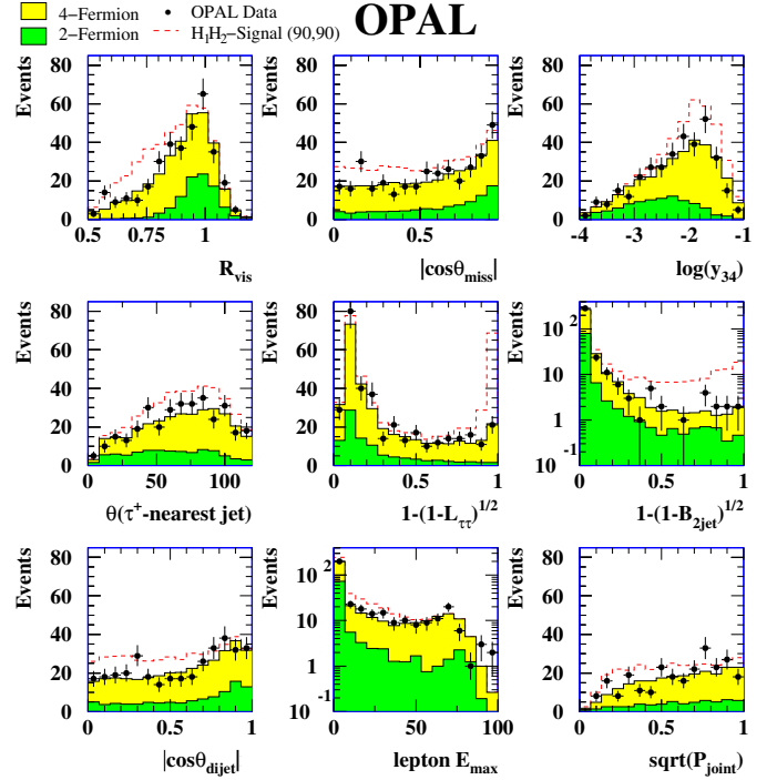
Fig. 10. Input variables [7] for the e^+e^- \rightarrow \mathcal{H}_1\mathcal{H}_2 \rightarrow \text{bb}\bar{\tau}^+\tau^- searches at 192–209 GeV
