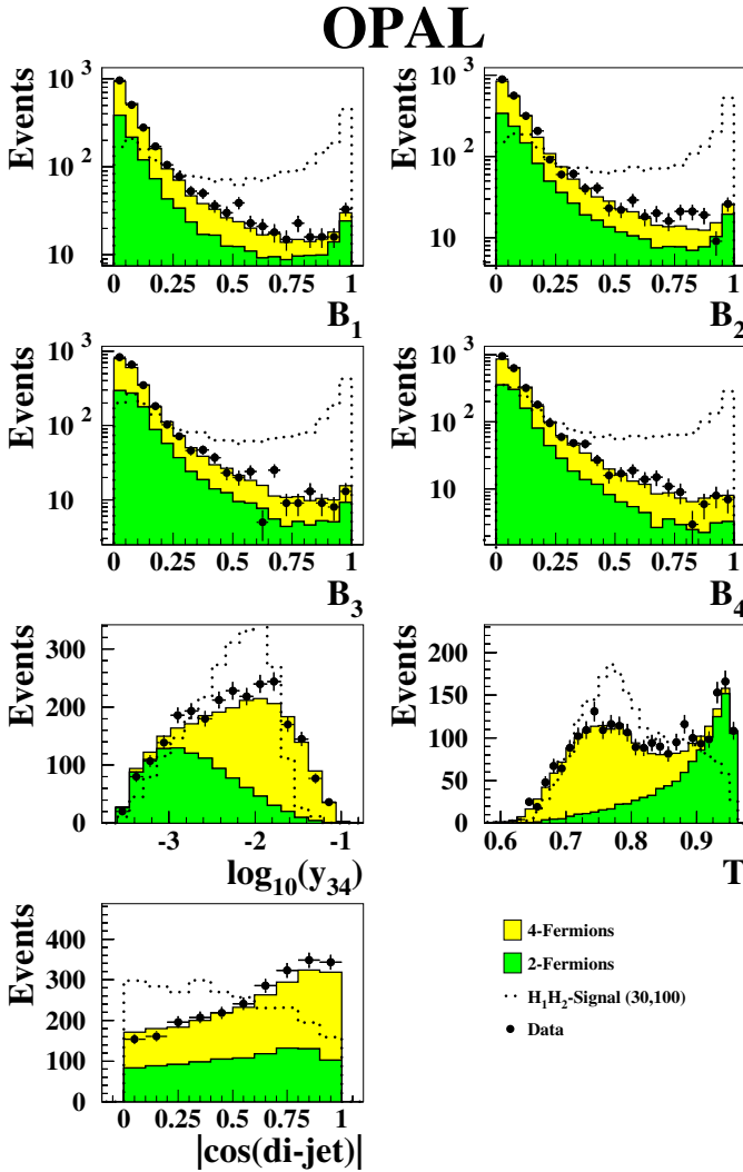
Fig. 6. Distributions of the input variables for the e^+e^- \rightarrow \mathcal{H}_1\mathcal{H}_2 \rightarrow b\bar{b}b\bar{b} searches for low m_{\mathcal{H}_1} at 199–209 GeV (see Sect. 4.2.2)
