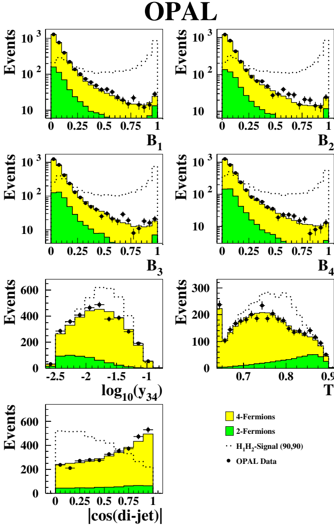
Fig. 5. Distributions of the likelihood input variables for the e^+e^- \rightarrow \mathcal{H}_1\mathcal{H}_2 \rightarrow b\bar{b}b\bar{b} searches for high m_{\mathcal{H}_1} at 192–209 GeV (see Sect. 4.2.1)
