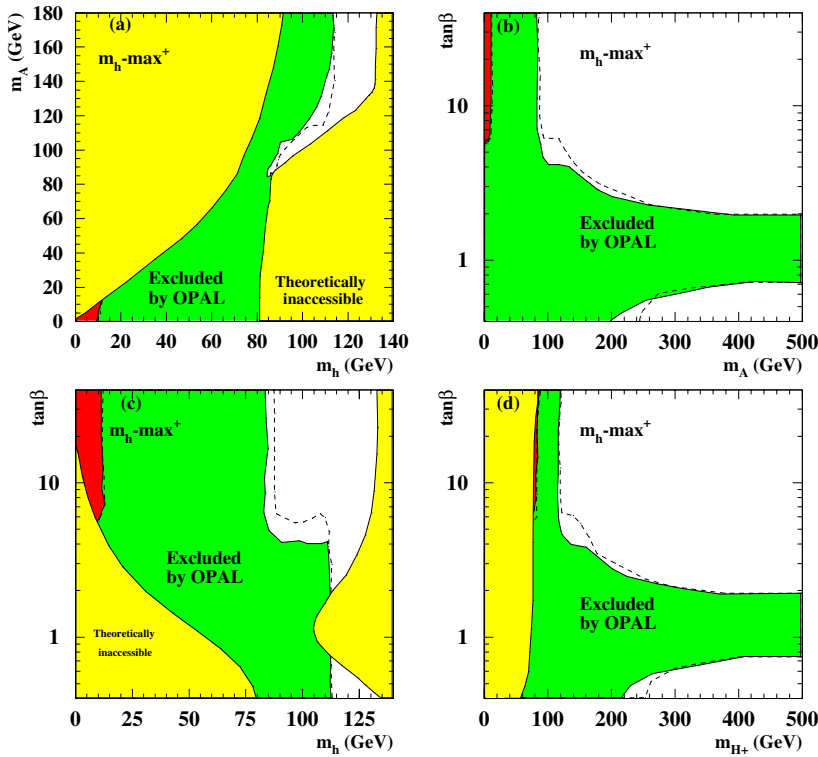
Fig. 17. Results for the m_h\text{-max}^+ benchmark scenario described in the text of Sect. 7.1. See Fig. 14 for the notation. This scenario is excluded by the \text{BR}(b\rightarrow s\gamma) constraint for m_A < 600 GeV
