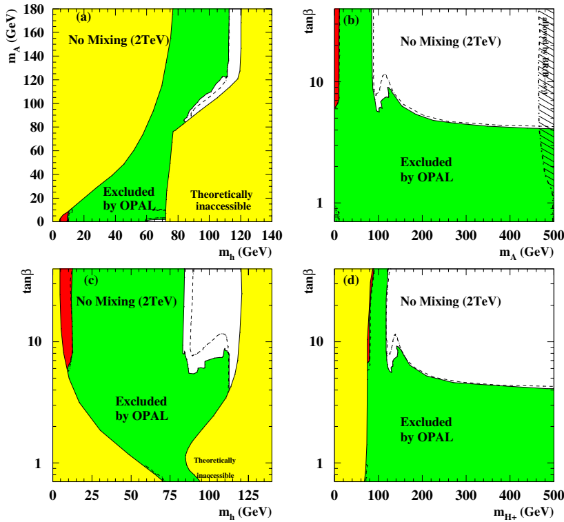
Fig. 15. Results for the no mixing (2 TeV) benchmark scenario described in the text of Sect. 7.1. See Fig. 14 for the notation
