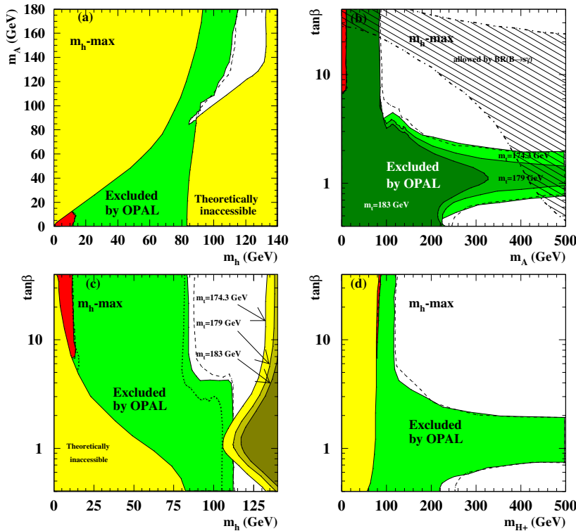
Fig. 16. Results for the m_h -max benchmark scenario. See Fig. 14 for the notation. The dotted line in c shows the observed 99.9% confidence limit. The differently shaded regions in b show the exclusion for different values of m_{top} , as written in the Plot. The upper limit on m_h for different values of m_{top} is shown in c , as expressed in the plot
