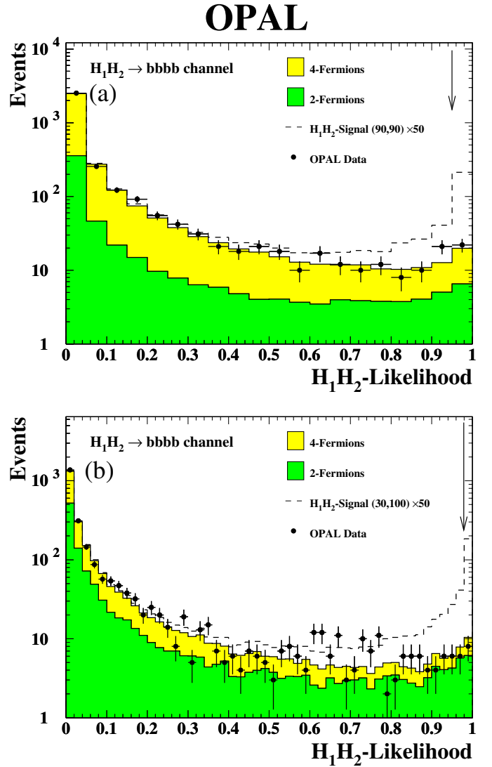
Fig. 7. Searches for e^+e^- \rightarrow \mathcal{H}_1\mathcal{H}_2 \rightarrow b\bar{b}b\bar{b} with high m_{\mathcal{H}_1} (see Sect. 4.2.1, 4.2.2) at 192–209 GeV. Likelihood outputs for a high m_{\mathcal{H}_1} , and b low m_{\mathcal{H}_1} . The arrow indicates the cut position. The signal is scaled with a factor of 50 with respect to a e^+e^- \rightarrow \mathcal{H}_1\mathcal{H}_2 \rightarrow b\bar{b}b\bar{b} signal for \cos^2(\beta - \alpha) = 1
