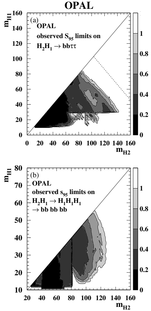
Fig. 13. Model-independent upper bounds on \sigma \times \text{BR} for a the e^+e^- \rightarrow \mathcal{H}_1 \mathcal{H}_2 \rightarrow b\bar{b}\tau^+\tau^- channel and b the e^+e^- \rightarrow \mathcal{H}_1 \mathcal{H}_2 \rightarrow \mathcal{H}_1 \mathcal{H}_1 \mathcal{H}_1 \rightarrow b\bar{b}b\bar{b}b\bar{b} channel. The MSSM cross-section for \mathcal{H}_1 \mathcal{H}_2 production with \cos^2(\beta - \alpha) = 1 is taken as normalisation. The dashed line indicates the kinematic limit for \sqrt{s} = 206 GeV
