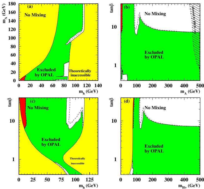
Fig. 14. Results for the no mixing benchmark scenario. The figure shows the excluded regions in darker grey (green) and theoretically inaccessible regions in light grey (yellow) as functions of the MSSM parameters in four projections: a the (m_h, m_A) plane, b the (m_A, \tan \beta) plane, c the (m_h, \tan \beta) plane and d the (m_{H^\pm}, \tan \beta) plane. The dashed lines indicate the boundaries of the regions expected to be excluded at the 95% CL if only SM background processes are present. The region excluded by Yukawa searches, Z-width constraints or decay independent searches is shown in dark grey (red). In b the hatched area is still allowed by \text{BR}(b \rightarrow s\gamma) searches
