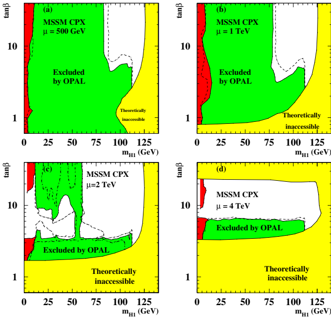
Fig. 27. The CPX MSSM 95 % CL exclusion areas in the (m_{H_1}, \tan\beta) plane, using scans with a \mu = 500 GeV, b \mu = 1000 GeV, c \mu = 2000 GeV (CPX) and d \mu = 4000 GeV. See Fig. 14 for the notation
