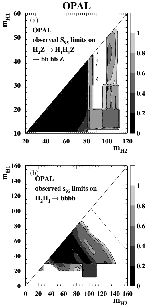
Fig. 12. Model-independent upper bounds on \sigma \times \text{BR} for a the e^+e^- \rightarrow \mathcal{H}_2 Z \rightarrow \mathcal{H}_1 \mathcal{H}_1 Z \rightarrow b\bar{b}b\bar{b}Z channel and b the e^+e^- \rightarrow \mathcal{H}_1 \mathcal{H}_2 \rightarrow b\bar{b}b\bar{b} channel. For a , the SM cross-section for \mathcal{H}_{\text{SM}}Z production is taken as normalization. For b , the MSSM cross-section for \mathcal{H}_1 \mathcal{H}_2 production with \cos^2(\beta - \alpha) = 1 is taken as normalization. The dashed line indicates the kinematic limit for \sqrt{s} = 206 GeV
