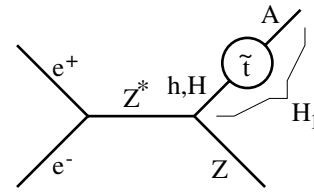
Fig. 22. Diagram illustrating the effective coupling of a Higgs mass eigenstate to the Z in Higgsstrahlung. The complete mass eigenstate \mathcal{H}_1 is composed of admixtures of h , H and A . Here the h , H and A denote the CP-even and CP-odd weak eigenstates, respectively. Only the CP-even admixtures h and H couple to the Z , while the CP-odd A does not. Therefore the coupling of the mass eigenstate is reduced with respect to a CPC scenario
