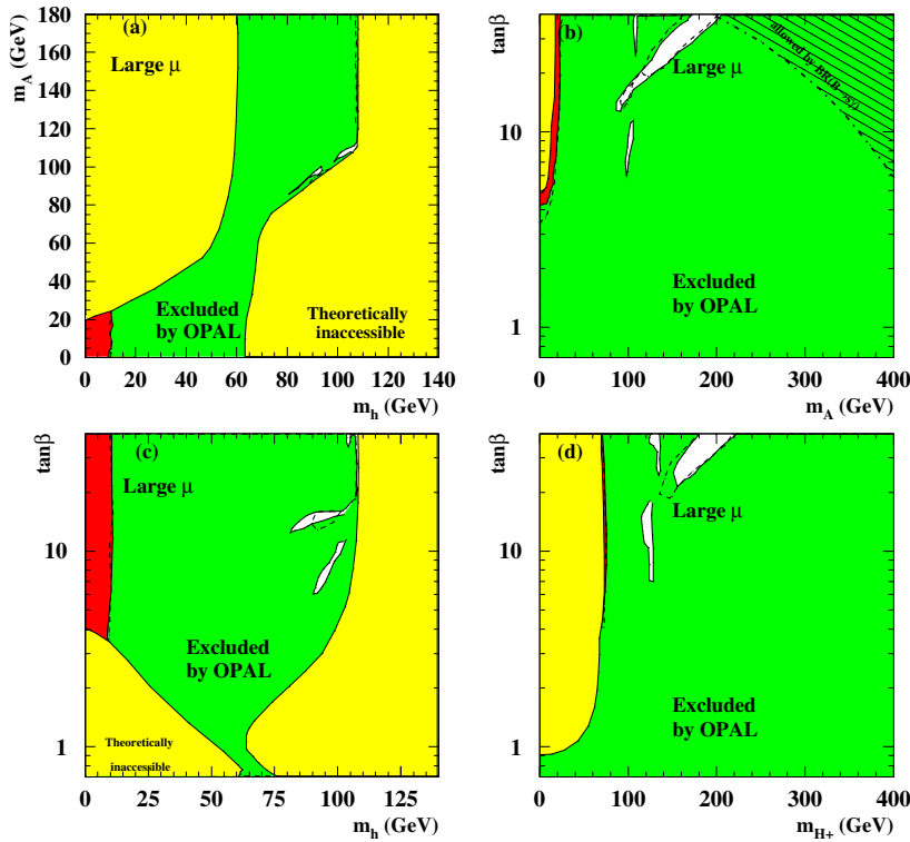
Fig. 19. Results for the large \mu benchmark scenario described in the text of Sect. 7.1. See Fig. 14 for the notation
