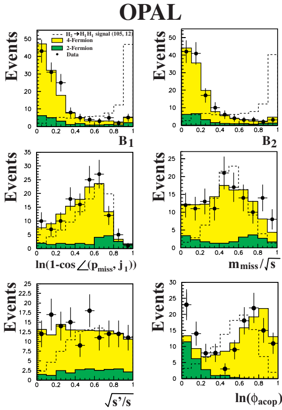
Fig. 1. Distributions of some ANN input variables for subsample A for e^+e^-\rightarrow\mathcal{H}_2Z\rightarrow b\bar{b}\nu\bar{\nu} and e^+e^-\rightarrow\mathcal{H}_1\mathcal{H}_1Z\rightarrow b\bar{b}b\bar{b}\nu\bar{\nu} (see Sect. 4.1.2) in the region 100 \text{ GeV} < m_{\mathcal{H}_2} < 110 \text{ GeV} for the data taken at \sqrt{s} = 199 - 209 GeV. Light grey (yellow) is the four-fermion background, dark grey (green) the contribution from the q\bar{q}(\gamma) background. The dashed line shows the arbitrarily scaled signal expectation for m_{\mathcal{H}_1} = 12 GeV and m_{\mathcal{H}_2} = 105 GeV, as given in the legend. The points with error bars are the data
